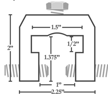
RoofClamp™ RCT
