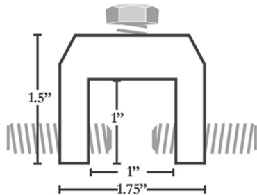
RoofClamp™ RC
